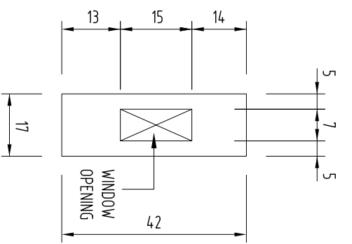
FIGURE 7 CORRIDOR WALL PARTITION TYPE C
