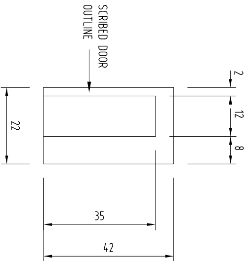
FIGURE 8 TOILET WALL PARTITION TYPE D
