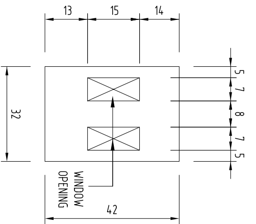
FIGURE 6 CORRIDOR WALL PARTITION TYPE B
